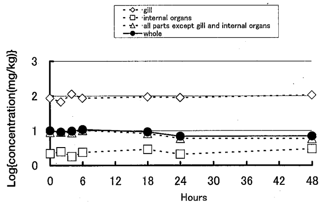
Fig3. Change of concentration of benzoepin in different organs of Ayu after exposing to 0.5mg/l benzoepin solution for half an hour
